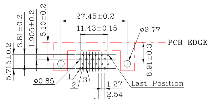
PCB Layout
