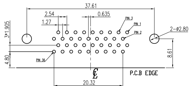
RECOMMENDED P.C.B LAYOUT INSPECTION DIMENSION:(A)~(H)
