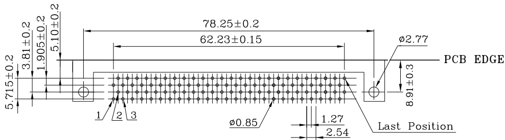
PCB Layout
