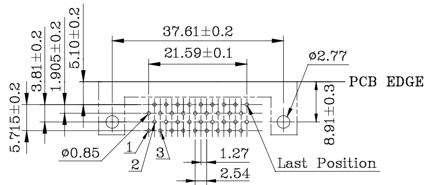
PCB Layout
