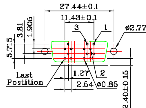
PC Board Mounting Dimensions
