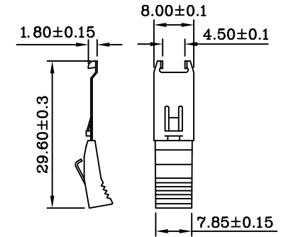
Flag Hooks
