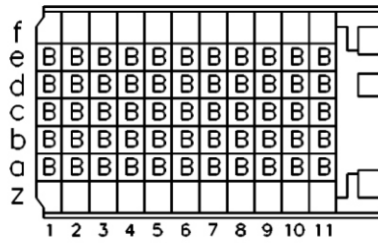
CONTACT LAYOUT
