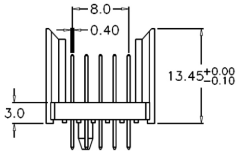
CONTACT LAYOUT
