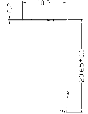
Top Shielded
