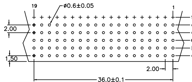
P.C. Board Layout (Top View)
