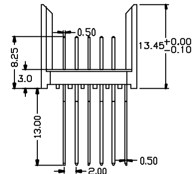
CONTACT LAYOUT
