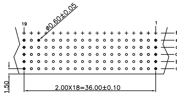
P.C. Board Layout (Top View)
