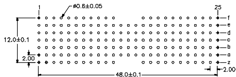
P.C. Board Layout (Top View)
