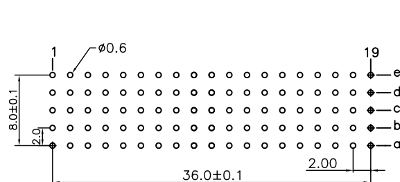
P.C. Board Layout (Top View)
