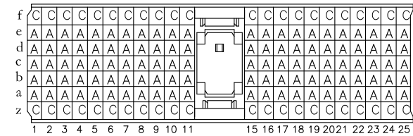
CONTACT LAYOUT
