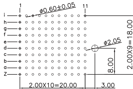
P.C. Board Layout (Top View)
