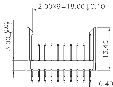
CONTACT LAYOUT
