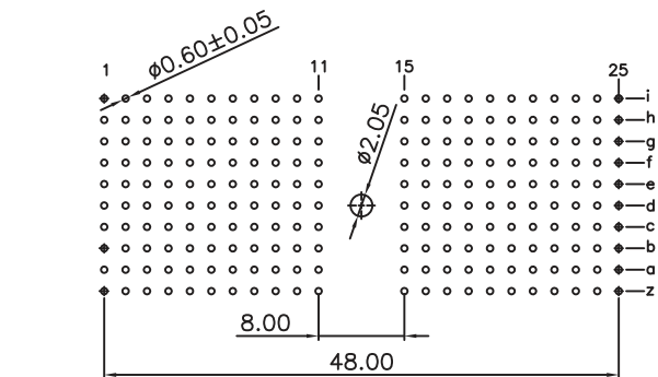
P.C. Board Layout (Top View)
