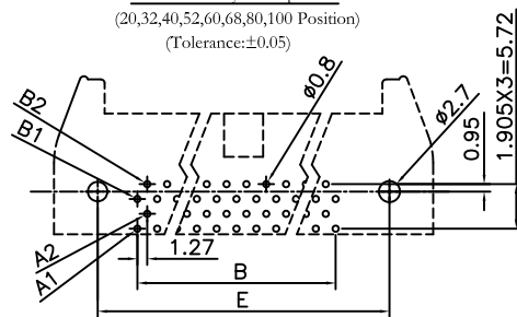
P.C. Board Layout Top View (26,34,50 Position) (Tolerance:±0.05)
