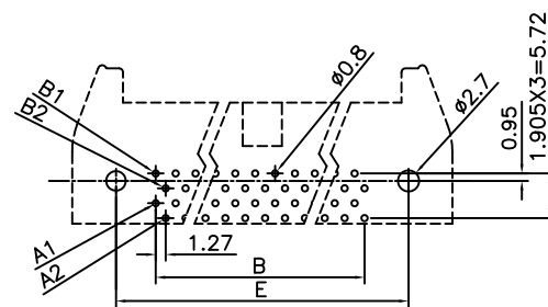
P.C. Board Layout Top View (20,32,40,52,60,68,80,100 Position) (Tolerance:±0.05)
