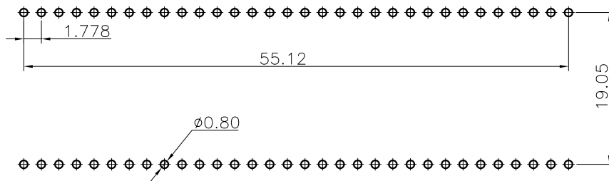
TOP VIEW PCB LAYOUT RECOMMENDED
