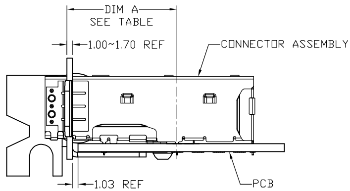
ASSEMBLED VIEW
