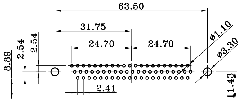
PCB LAYOUT
