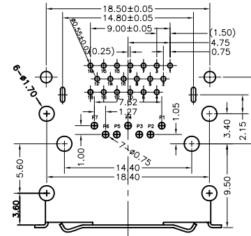
RECOMMENDED PCB LAYOUT (THICKNESS=1.6±0.15mm)
