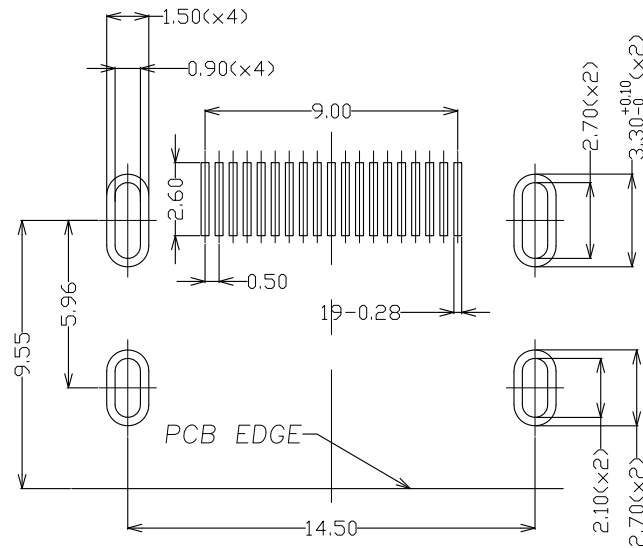
RECOMMENDED P.C.B LAYOUT (THICKNESS=1.60±0.05mm)
