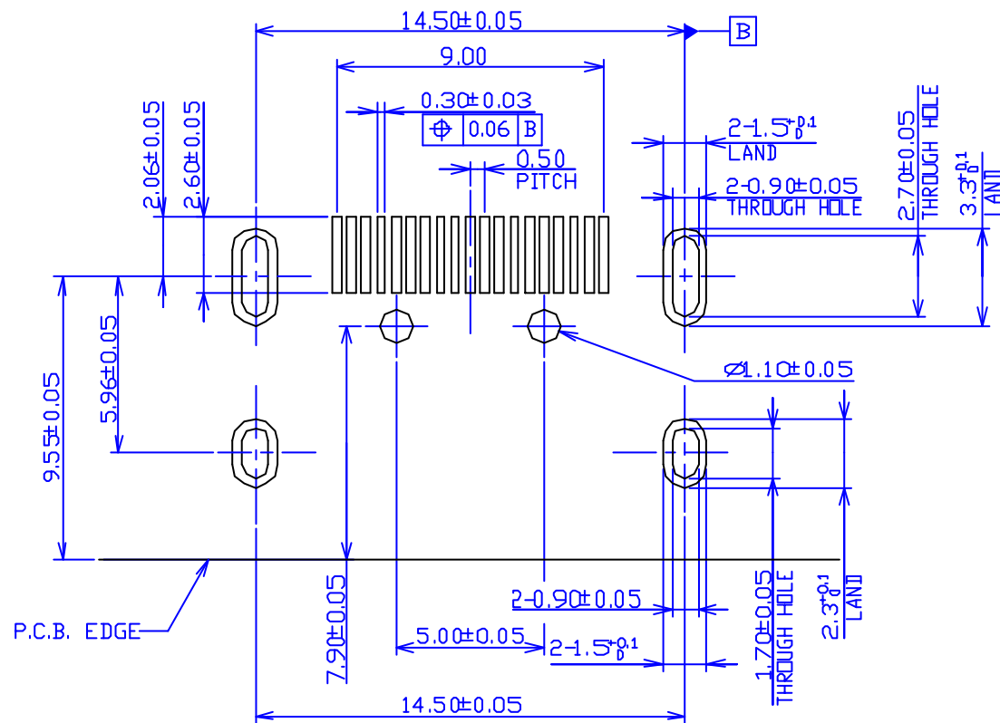
FIGURE A: Printed Circuit Board (PCB) Layout
