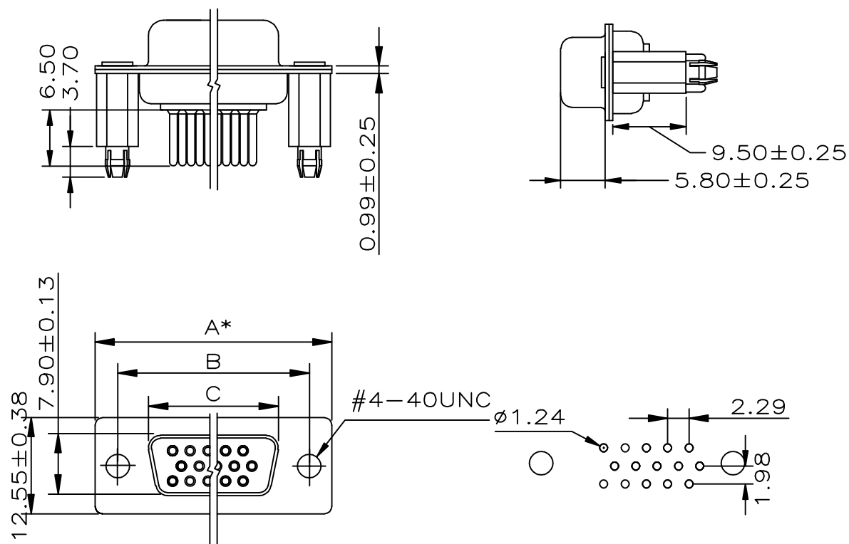
PCB LAYOUT
