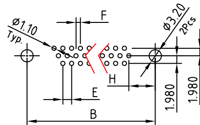
Re Layout P.C.B. 26 /44 /62POSITION
