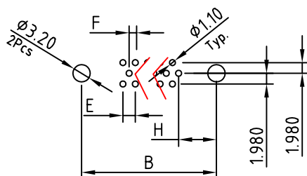
Re Layout P.C.B. 15 POSITION
