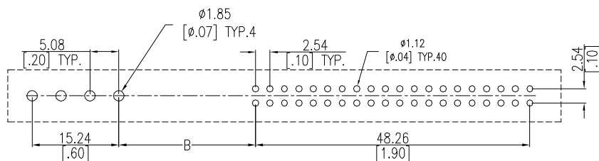
PCB LAYOUT
