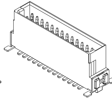
STANDING HEIGHT: B (8.25) HAUB-PV32P-xxx
