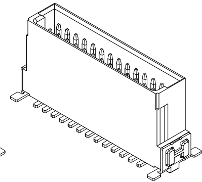
STANDING HEIGHT: C (9.85) HAUB-PV48P-xxx
