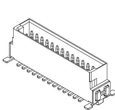
STANDING HEIGHT: A (6.75) HAUB-PV17P-xxx
