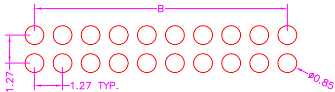
P.C.B. LAYOUT TOP VIEW ±0.05
