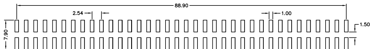
Recommended P.C.B Layout
