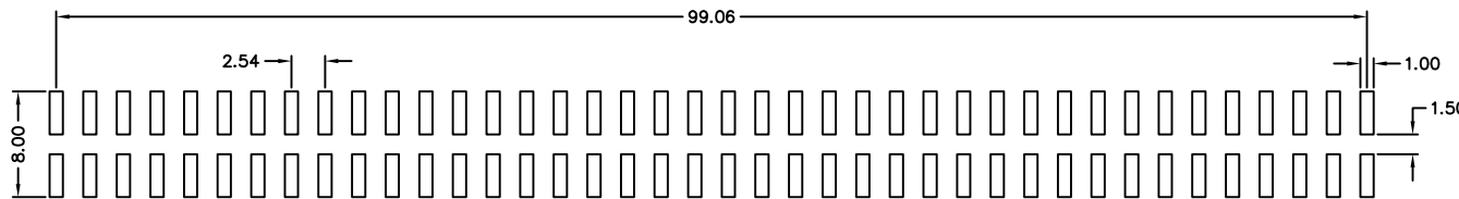
Recommended P.C.B Layout
