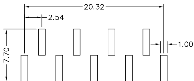
B-TYPE Recommended P.C.B Layout
