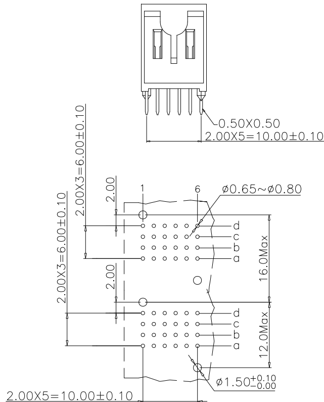
P.C. Board Layout
