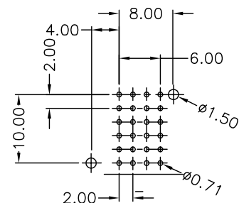
Solder pin
