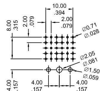
Recommended P.C Board Hole Layout
