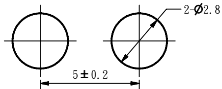
MOUNTING HOLES
