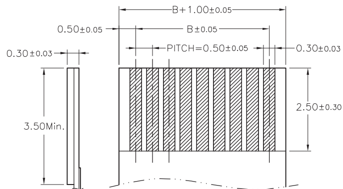
APPLICABLE FPC
