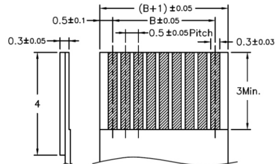
Applicable FPC
