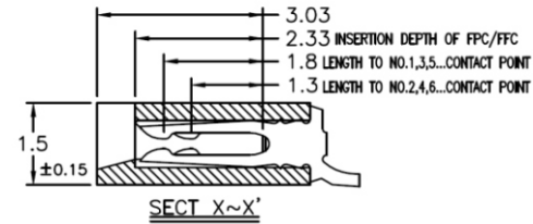
Applicable FPC
