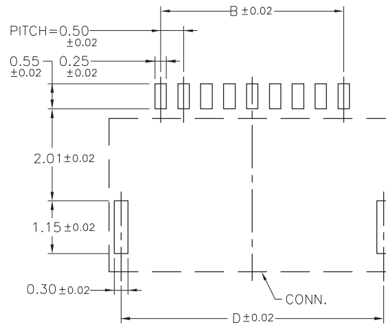
RECOMMENDED METAL MASK PATTERN(THICKNESS 0.1mm)
