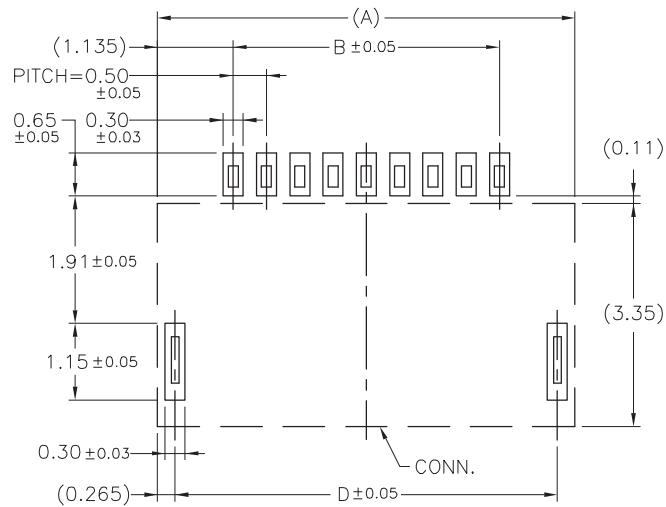
FPC/FFC INSERT DIRECTION PCB LAYOUT
