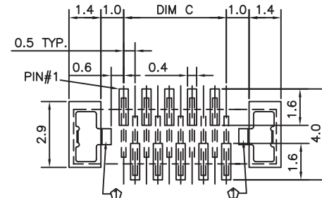
RECOMMENDED PCB LAYOUT(EVEN PIN) GENERAL TOLERANCE \pm 0.05
