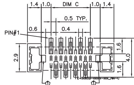
RECOMMENDED PCB LAYOUT(ODD PIN) GENERAL TOLERANCE \pm 0.05
