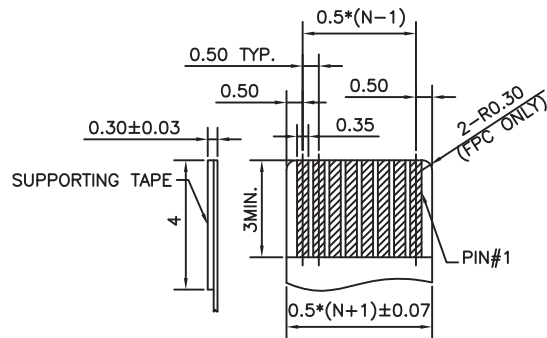
APPLICABLE FPC/FFC LAYOUT GENERAL TOLERANCE \pm 0.05
