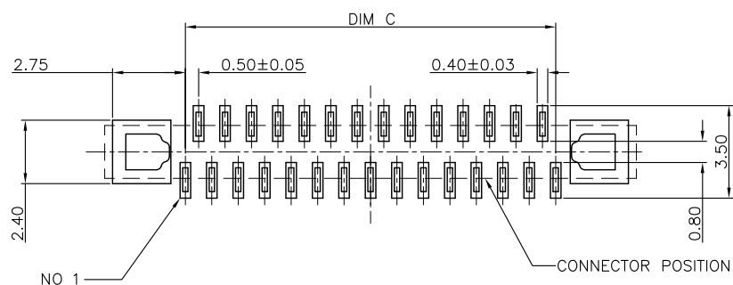
Positive PCB LAYOUT
