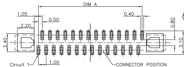
RECOMMENDED P.C.B PATTERN LAYOUT
