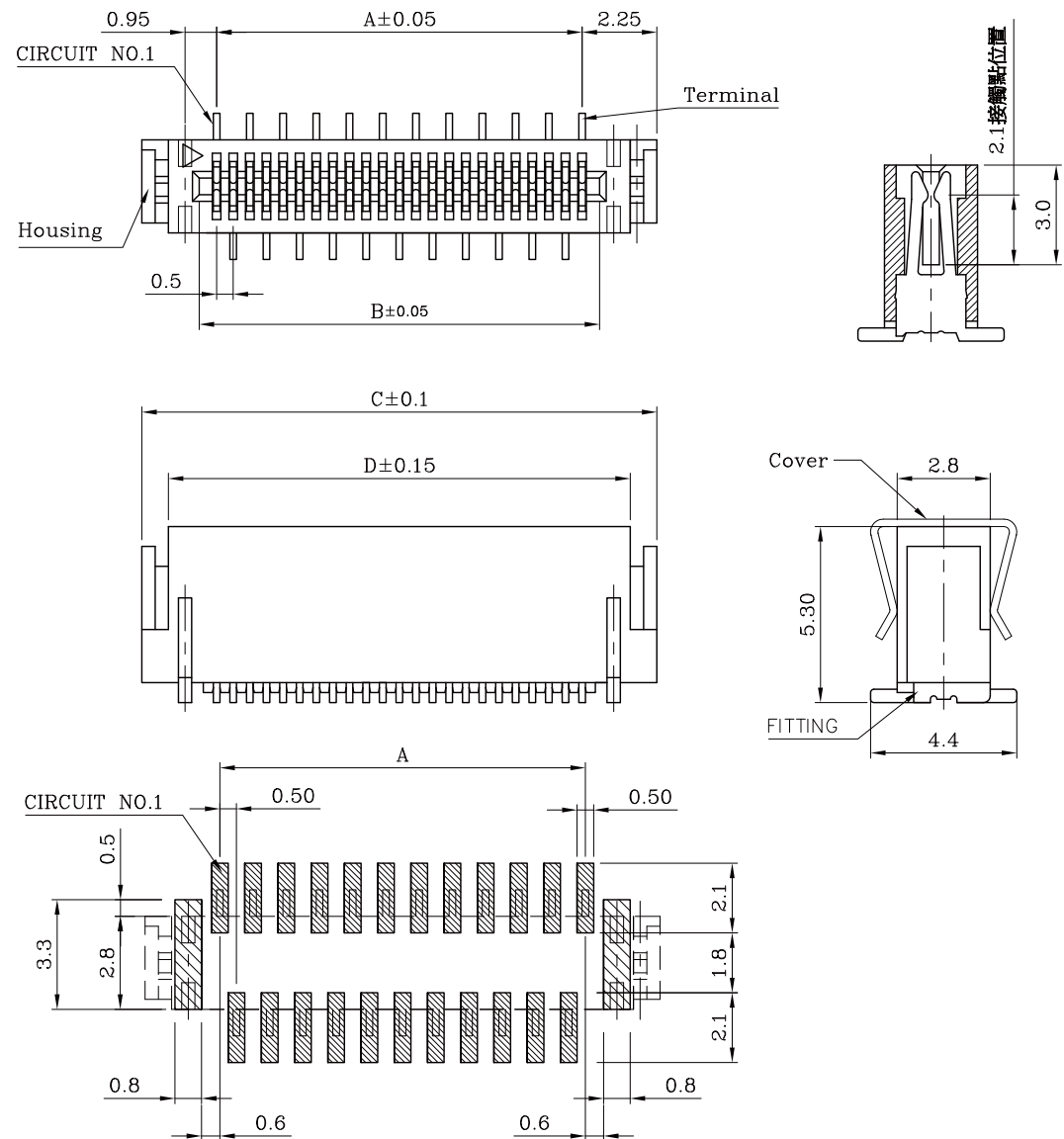
PC. BOARD LAYOUT
