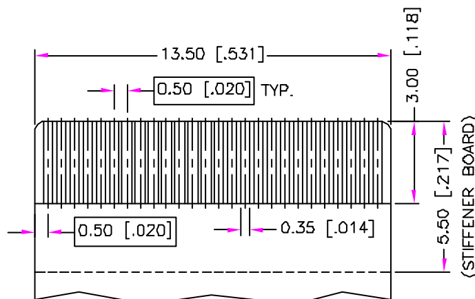
APPLICABLE FPC RECOMMEND DIMENSION (t=0.30mm)
