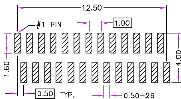
RECOMMEND P.C.B. LAYOUT TOP VIEW
