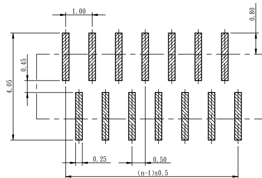
REFERENCE PCB PATTERN
