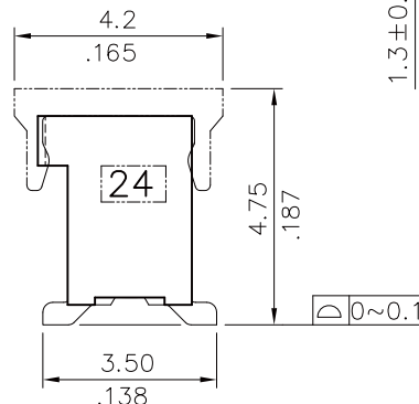
DETAIL "A-A"
