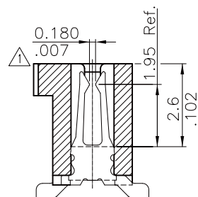
DETAIL "A-A"
