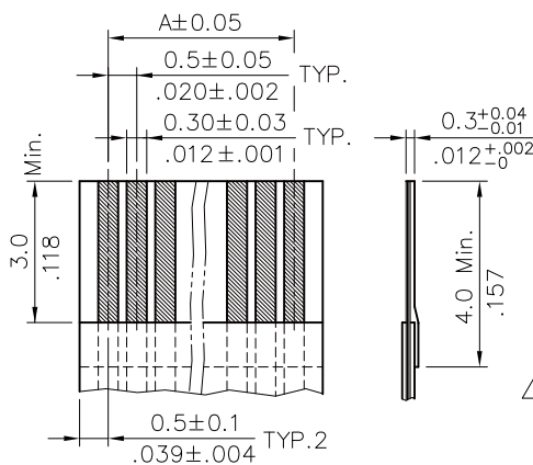
Accommodated FFC/FPC
