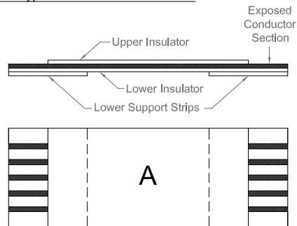
Cable Type A - Conductor Same Side
