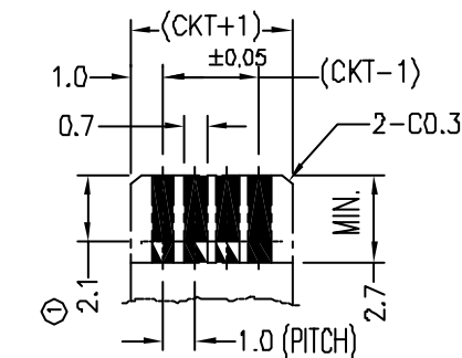
RECOMMENDED APPLICABLE FPC LAYOUT
