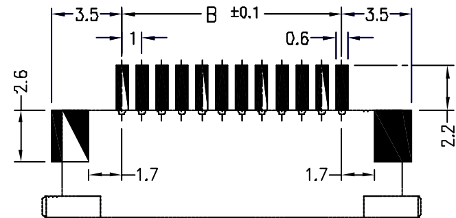
RECOMMENDED PATTERN DIM. (REF.)
