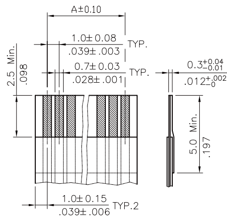
Accommodated FFC/FPC
