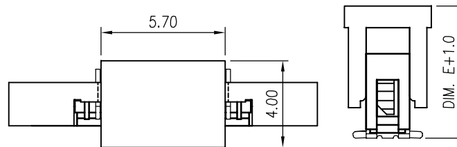
CAP PLACEMENT DIAGRAM
