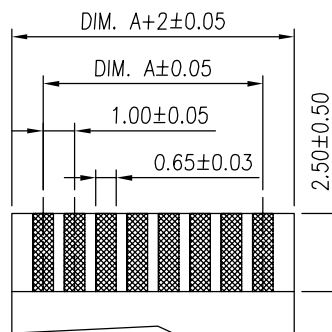
FFC/FPC DIMENSION THICKNESS 0.30 \pm 0.03 mm
